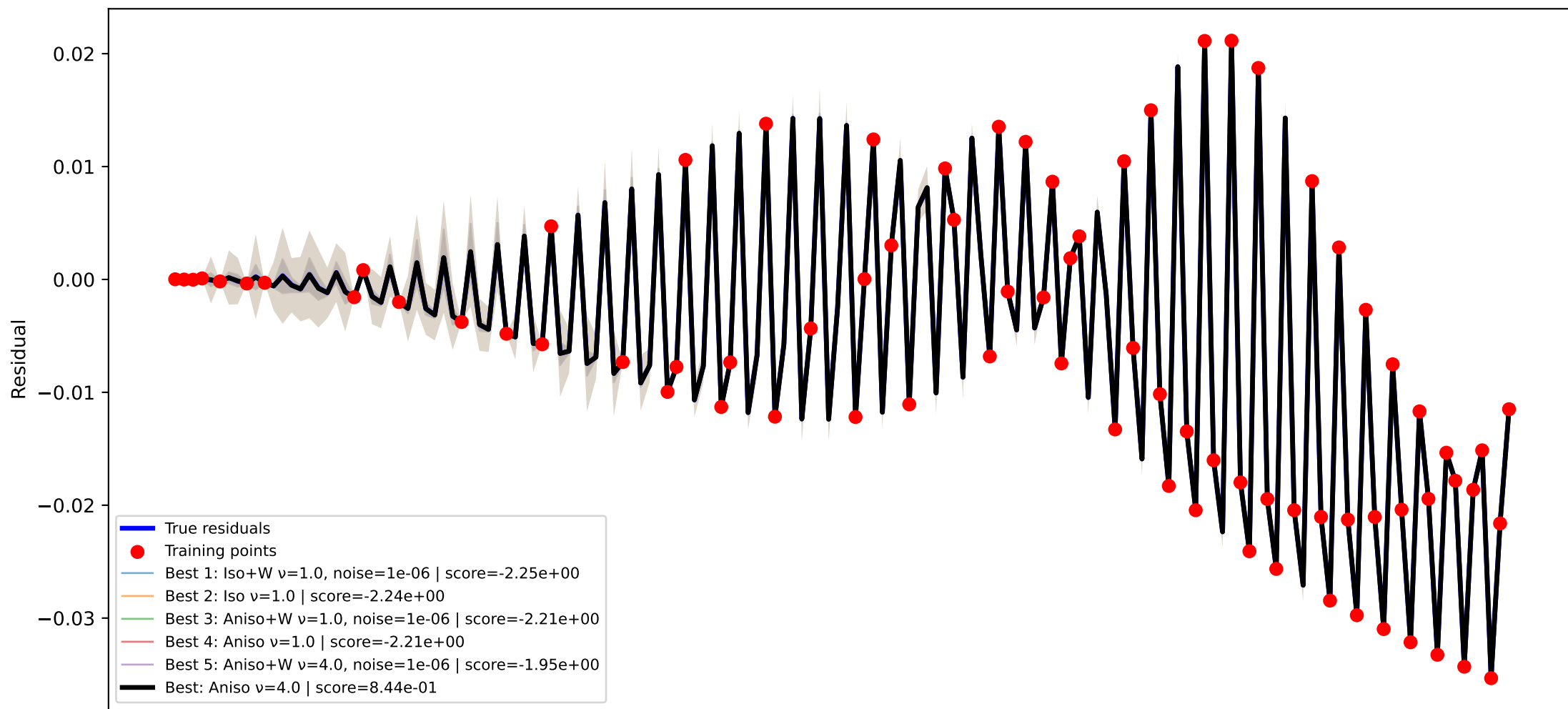
GPR kernel comparison node=8 RMSE=1.243e-05, train RMSE=4.831e-10
